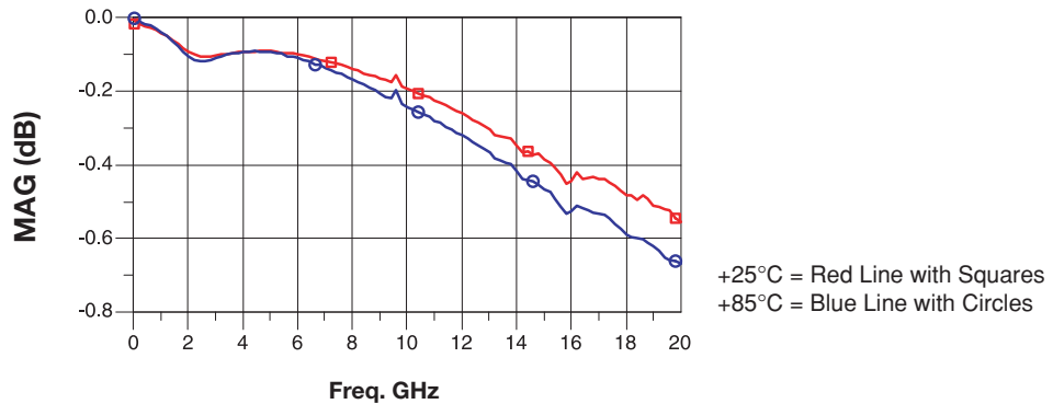
Transmission Loss Over Temperature (S21)
